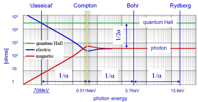
FIG. 1. Photon and electron impedances as a function of spatial scale as defined by photon energy. The role of the fine structure constant \alpha in the impedance and energy ratios is a prominent feature of the figure.
