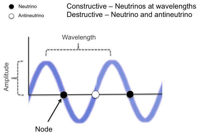
Figure 2 – Neutrino and Antineutrino Placement
