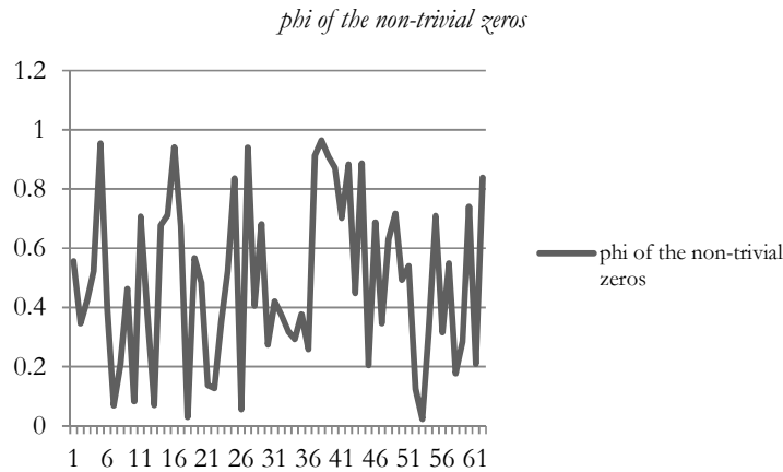
Figure 1 , graph of \hat{\phi}_{\sigma_\rho}(\omega_\rho) over its corresponding positive integer
