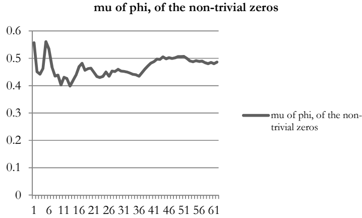
Figure 2, graph of \mu of \hat{\phi}_p(\omega_p) over its corresponding positive integer
