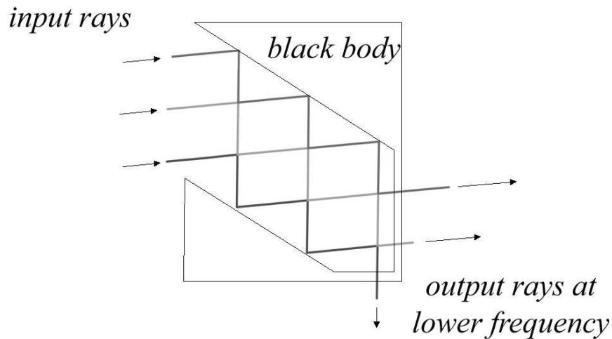
Figure 6, black body representation of \hat{\phi}_{1/3}(N) in terms of Rayleigh scattering
