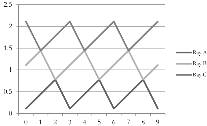
Figure 5, graph of \hat{\phi}_{1/3}(N) and two multiplicative factors over the natural numbers
