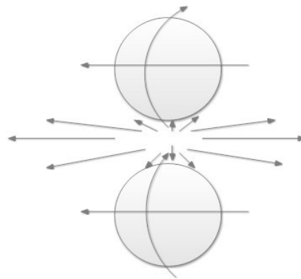
Repulsion
