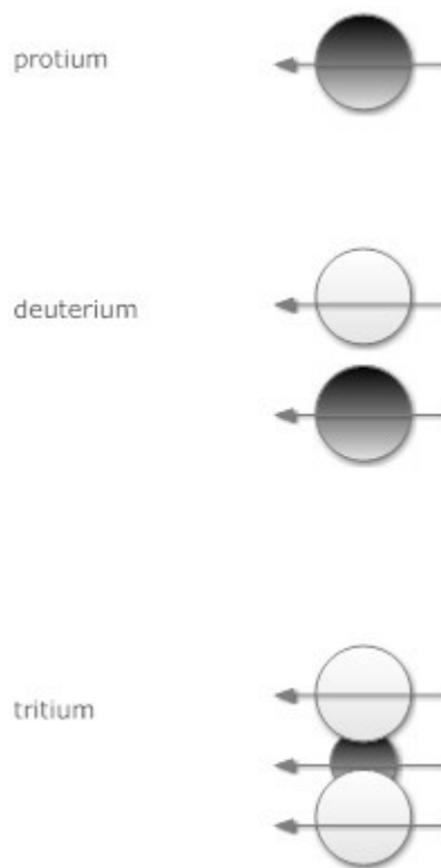
Hydrogen isotopes
