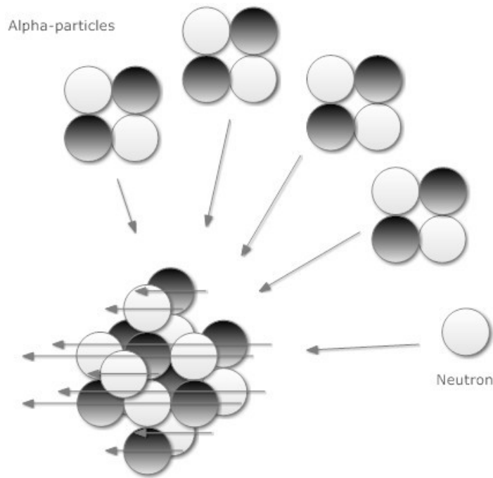
Oxygen-17
