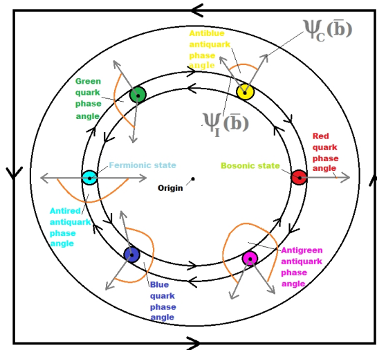
FIG. 10: Leggett's [71] six distinct superfluid B phase angles for the three q\bar{q} pairs confined to T along the six-coloring kagome lattice of antiferromagnetic ordering [4, 38]. The superfluid B phase angles \langle r \rangle, \langle g \rangle, \langle b \rangle, \langle \bar{r} \rangle, \langle \bar{g} \rangle, \langle \bar{b} \rangle remain constant and correlate the OPs as they rotate freely in 2D and 3D space; this long range order applies \forall t \in T, \forall \psi \in \Phi_{OP} , to form correlated helices along T ; this concept serves as a strong WBWF constraint and applies to all OPs for a given time-point. In this diagram, only \psi_C(t) and \psi_I(t) are shown, but \psi_J(t) is also correlated with \langle t \rangle .
