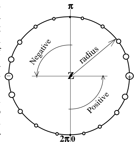
Fig. 3 HEM-HC Cylindrical Electric Field - Vertical View
