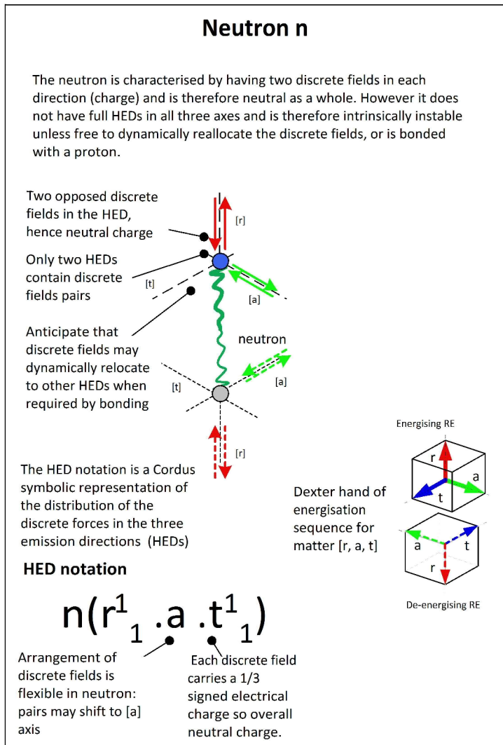
Figure 5: Cordus theory for the neutron. The distinguishing feature of this particule compared to the proton is the balanced number of inwards and outwards discrete forces, hence neutral charge.
