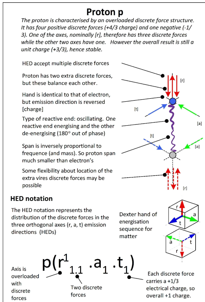
Figure 4: Cordus theory for the proton. The distinguishing feature of this particule is the overloaded discrete forces. The higher mass of the particule, compared to say the electron, is proposed to arise from the higher frequency of re-energisation for this particule, in turn driven by internal fibril dynamics not apparent here.
