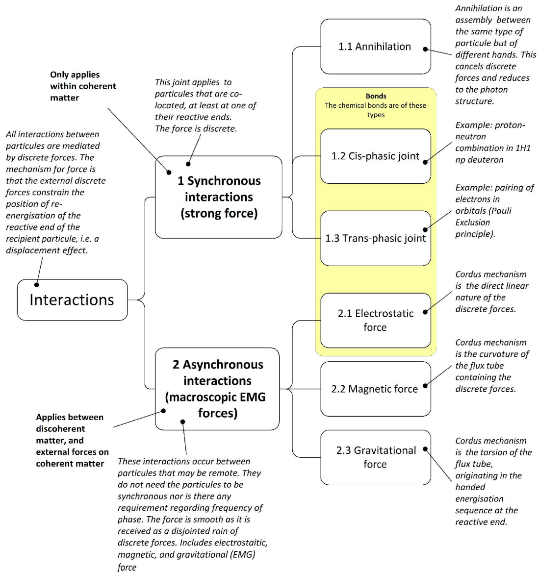
Figure 7: Cordus force hierarchy theory. All interactions between particules are mediated by discrete forces. The mechanism for force is that the discrete forces constrain the position of re-energisation of the reactive end of the recipient particule, i.e. a displacement effect. The state of the particules, particularly the synchronicity and phase of their frequency, results in several types of forces/interactions as shown.
