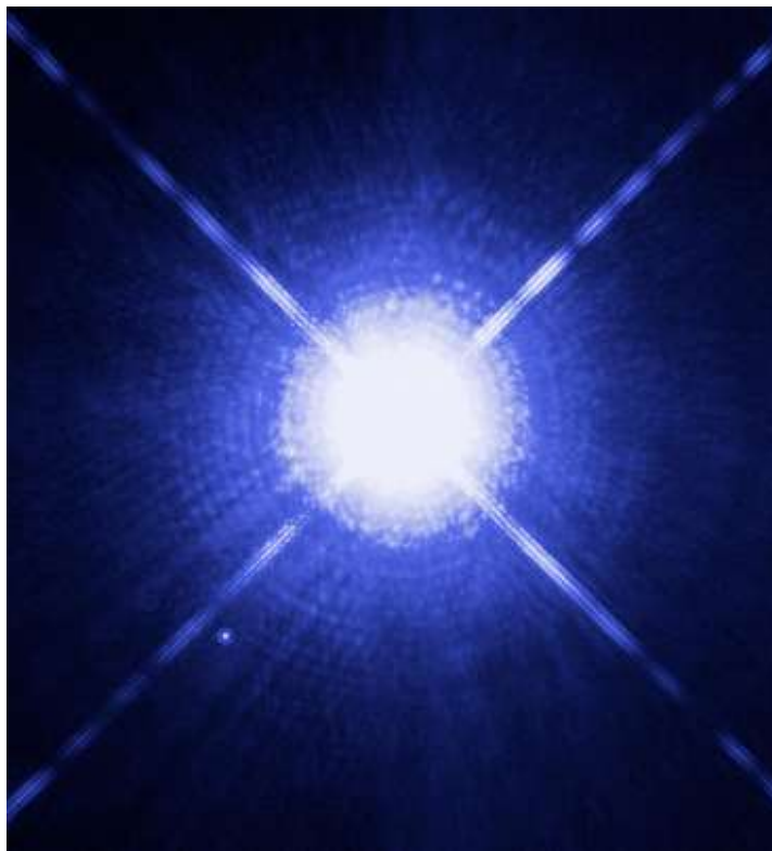
This image of Sirius A and Sirius B was taken Oct. 15, 2003, with Hubble's Wide Field Planetary Camera 2. WFPC2 NASA.
