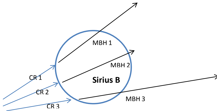
A diagram of CR collision with Sirius B (radius 5,842km) at various approach angles: Regardless of approach angle, an MBH product would typically require to traverse far longer than the calculated stopping distance of 1.5 km.
