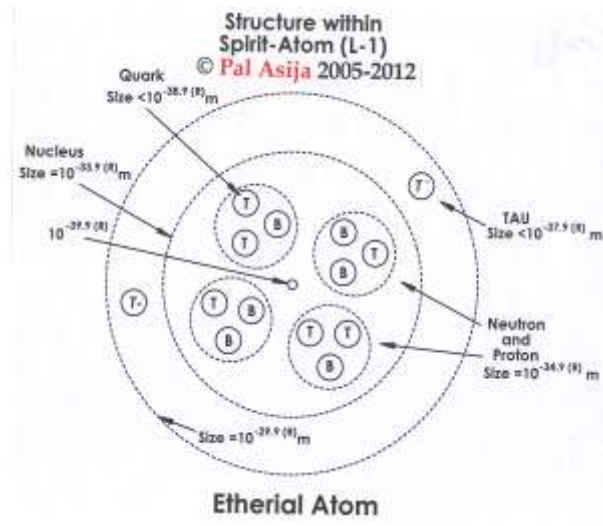
Fig. 5c Ethereal Atom Up Close
