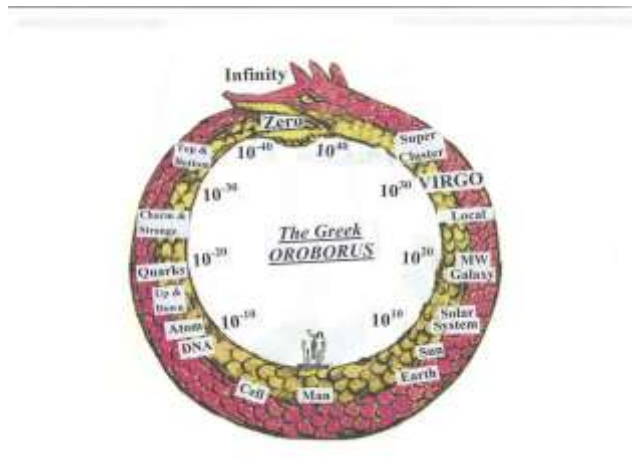
Fig. 3c. The Greek Oroborus
