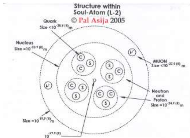
Fig. 5b Meta-Physical Atom Up Close
