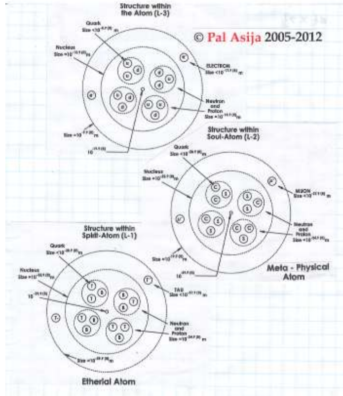
Fig. 5.0 Sub-meter scale Tri-level Atomic Structures
