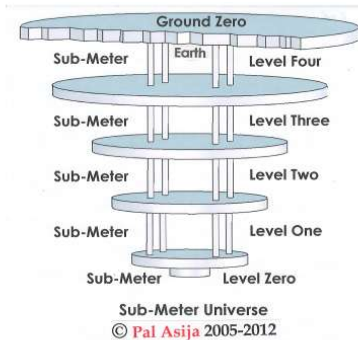
Fig. 3b. The Submeter Universe
