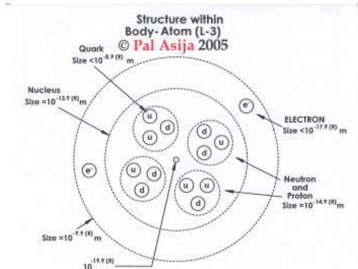
Fig. 5a Conventional Atom Up Close
