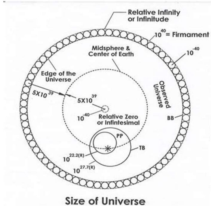
Fig.4c. Uniform Gravity Globe
