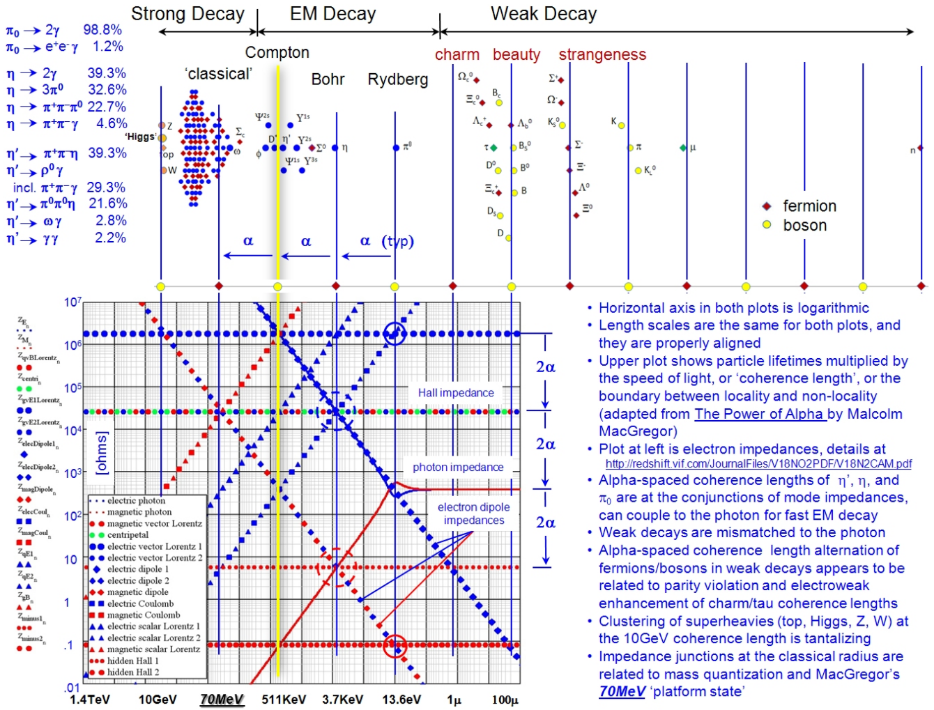
FIG. 2. A composite of 13.6eV photon impedances[8] and a variety of background independent[1]electron impedances[2, 6], measured branching ratios of the \pi_0 , \eta , and \eta' , the four fundamental quantum lengths shown in fig.1, and the coherence lengths of the unstable particles. Regarding dipole impedances, only the transverse dipole-dipole impedances are shown. Missing are the longitudinal dipole-dipole and longitudinal and transverse charge-dipole impedances.
