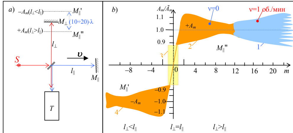
Fig.1. The scheme explaining effect of "spasmodic" change of a sign of amplitude of harmonious shift of a fringe interference by MI, which observed in a telescope ( T ), in the process of precisions adjustment by the micrometric screw of position of mirror M_{\parallel} in a longitudinal arm l_{\parallel} .
