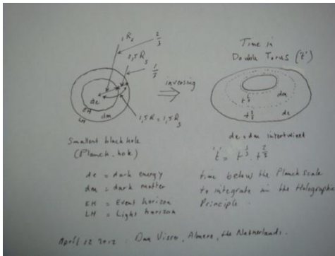
Fig. 2: A Double Torus geometry fundamentally follows from equations in publications [2] .
