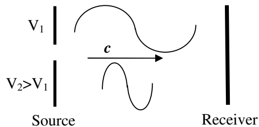
Figure 1 – Wavelength Contraction
