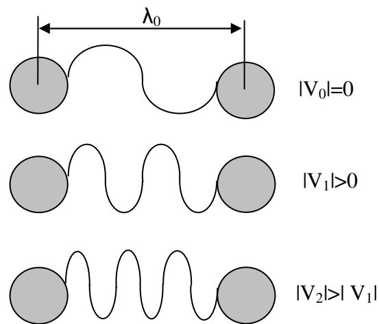
Figure 3 – The Relativistic Doppler Effect
