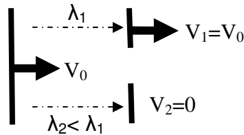
Figure 2 – Apparent ‘Slowing of Time’ in Special Relativity
