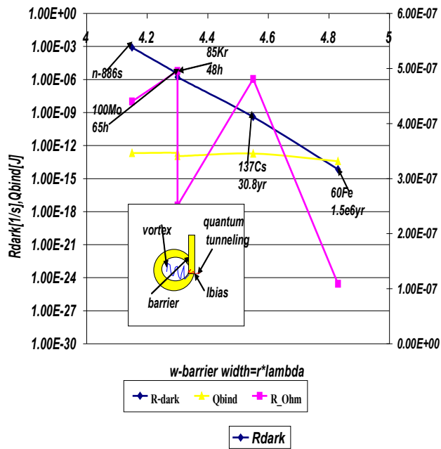
Fig.5. The evolution of dark count ( \beta decay) rate as function of barrier width.
