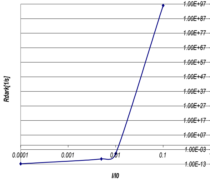
Fig.6 The evolution of the dark count rate ( \beta ) decay as a function of the bias current.
