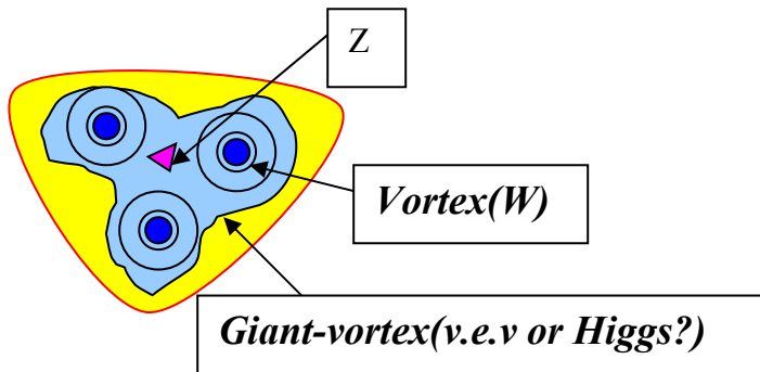
Fig.1b. The Giant-Vortex type arrangement for the nucleon
