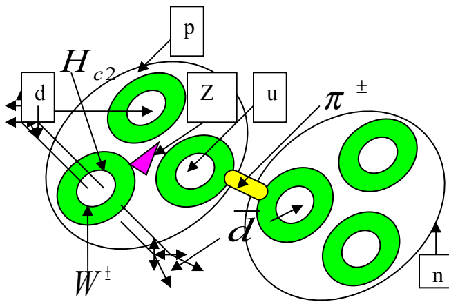
Fig.1a. Abrikosov’s triangular lattice for a nucleon (proposal)
