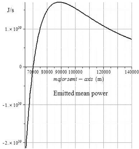
Fig. 3: Emitted mean power for Vortex model according to equ.(29), much lower than Einstein's amounting to 10E48.
