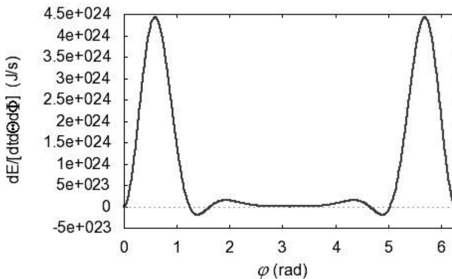
Fig. 4(b): Einstein's differential energy loss: 2\pi periodic emitted instantaneous power at given direction for Einstein's model at polar angle \Theta = \pi/2 and azimuth \Phi = \pi/2 .
