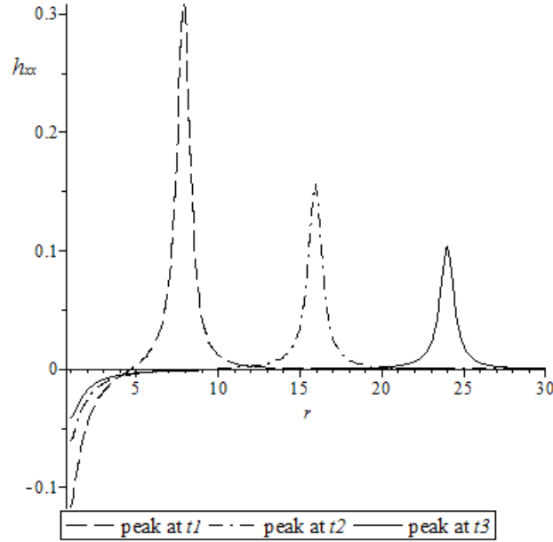
Fig1: Plot in function of r (arbitrary units) of the characteristic gravitational billow wave shape solution (numerical) h_{xx} with respect to a discontinuity source located about r=0 at fixed times t1 < t2 < t3 with its attenuating moving peak at r = ct .
