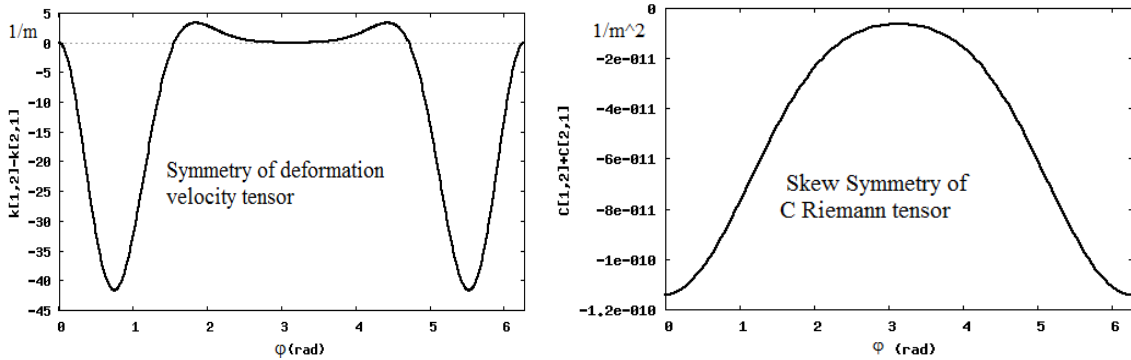
Fig 2: Plot in function of the azimuthal angle along the elliptic orbit of the approximation precision K_{12} - K_{21} and C_{12} + C_{21} respectively.
