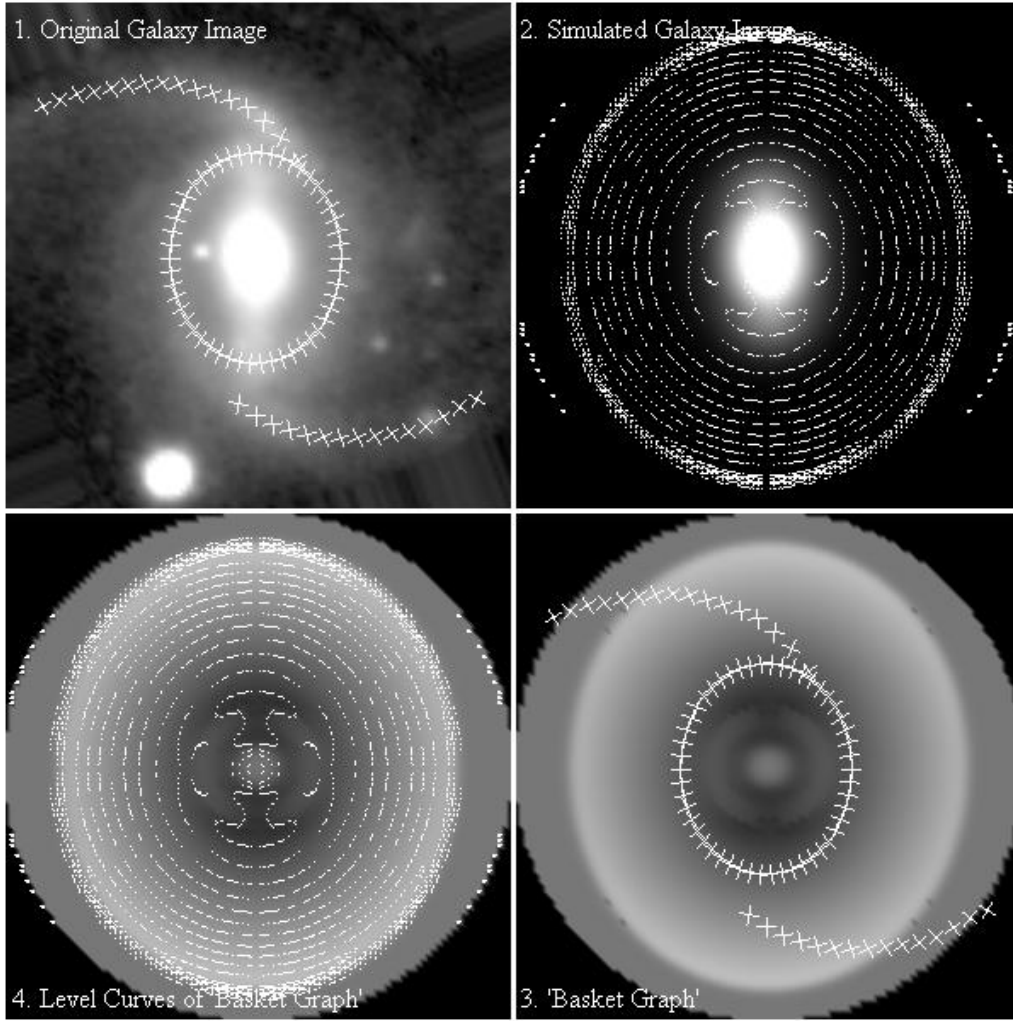
Figure 3: Upper left is a longer-wavelength image of barred spiral galaxy NGC 5921 (see [6] for image credit). Upper right is its simulation with an exponential disk and two dual-handle structures. Lower right is its ‘basket graph’ which is a demonstration of the function u(x, y) with the image brightness at each point being proportional to the corresponding value of the function. The function is the variance rate of f(x, y) along the direction of \alpha that is solved from instinct equation. Lower left is the level curves of u(x, y) which are simultaneously the proportion curves of barred galaxy. The curves are spider-shaped.
