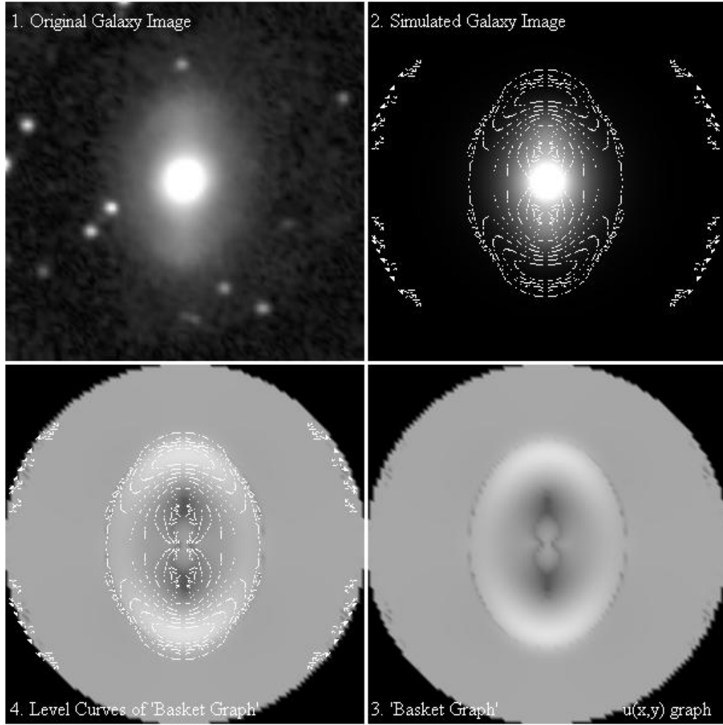
Figure 3: Upper left is a longer-wavelength image of barred spiral galaxy NGC 6782 (see [?] for image credit). Upper right is its simulation with an exponential disk and two dual-handle structures. Lower right is its ‘basket graph’ which is a demonstration of the function u(x, y) with the image brightness at each point being proportional to the corresponding value of the function. The function is the variance rate of f(x, y) along the direction of \alpha that is solved from instinct equation. Lower left is the level curves of u(x, y) which are simultaneously the proportion curves of barred galaxy. The curves are spider-shaped.
