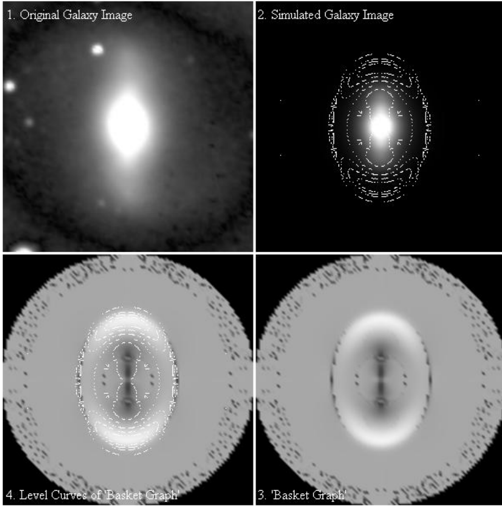
Figure 3: Upper left is a longer-wavelength image of barred spiral galaxy NGC 4665 (see [6] for image credit). Upper right is its simulation with an exponential disk and two dual-handle structures. Lower right is its ‘basket graph’ which is a demonstration of the function u(x, y) with the image brightness at each point being proportional to the corresponding value of the function. The function is the variance rate of f(x, y) along the direction of \alpha that is solved from instinct equation. Lower left is the level curves of u(x, y) which are simultaneously the proportion curves of barred galaxy. The curves are spider-shaped.
