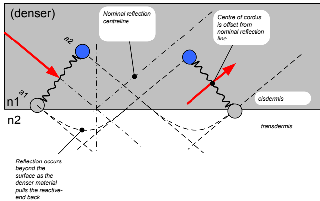
Figure 5: Reflection occurs as a curved transition some distance off the surface (a), not an abrupt change at the precise surface. In the case of internal reflection (b), the transition may occur in the second medium and result in the centre of the cordus being offset from the nominal.
