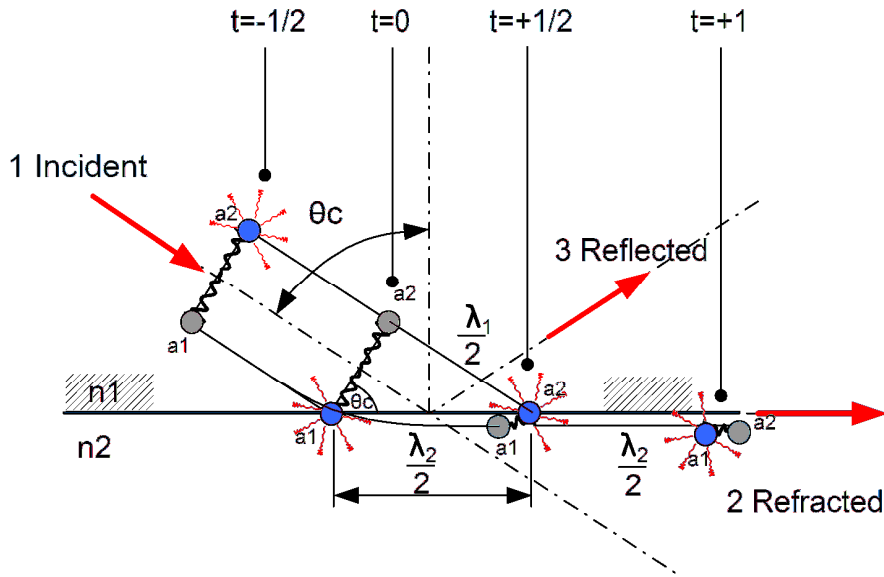
Figure 6: Geometry of the cordus at the critical angle \vartheta_c for total internal reflection.
