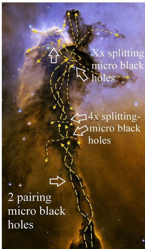
Figure 10, Comparison with splitting and pairing Micro black holes inside Planetary nebula, and the formation of comet nuclei like the Hyperion icy nucleus.
