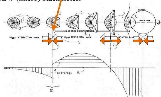
Figure 10, Comparison with splitting and pairing Micro black holes inside Planetary nebula, and the formation of comet nuclei like the Hyperion icy nucleus.
