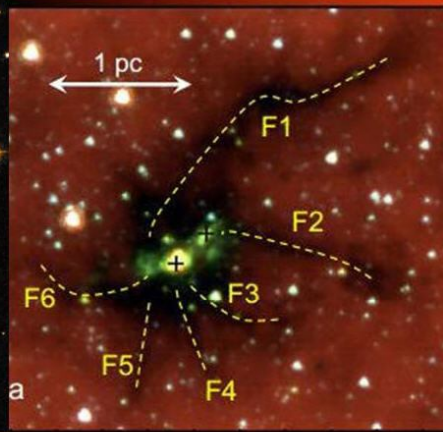
SDC 335 with gas filaments as multiple Herbig Haro objects
