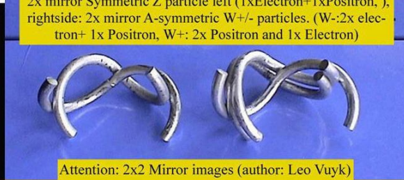
The alternative standard model with some 3-D examples of different particles?
