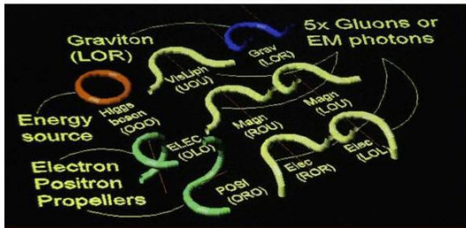
The alternative standard model with some 3-D examples of different particles?
