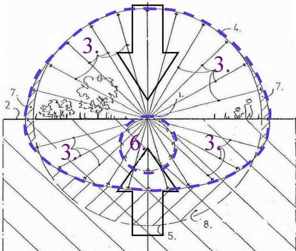
Figure 6, Cross section of the “Double Vector Hedgehog” of pushing forces around Fermions. The difference between Higgs vacuum pressure (3) and less effective Graviton pressure (6) on Fermions are the basic elements of Double Le Sage gravity.
