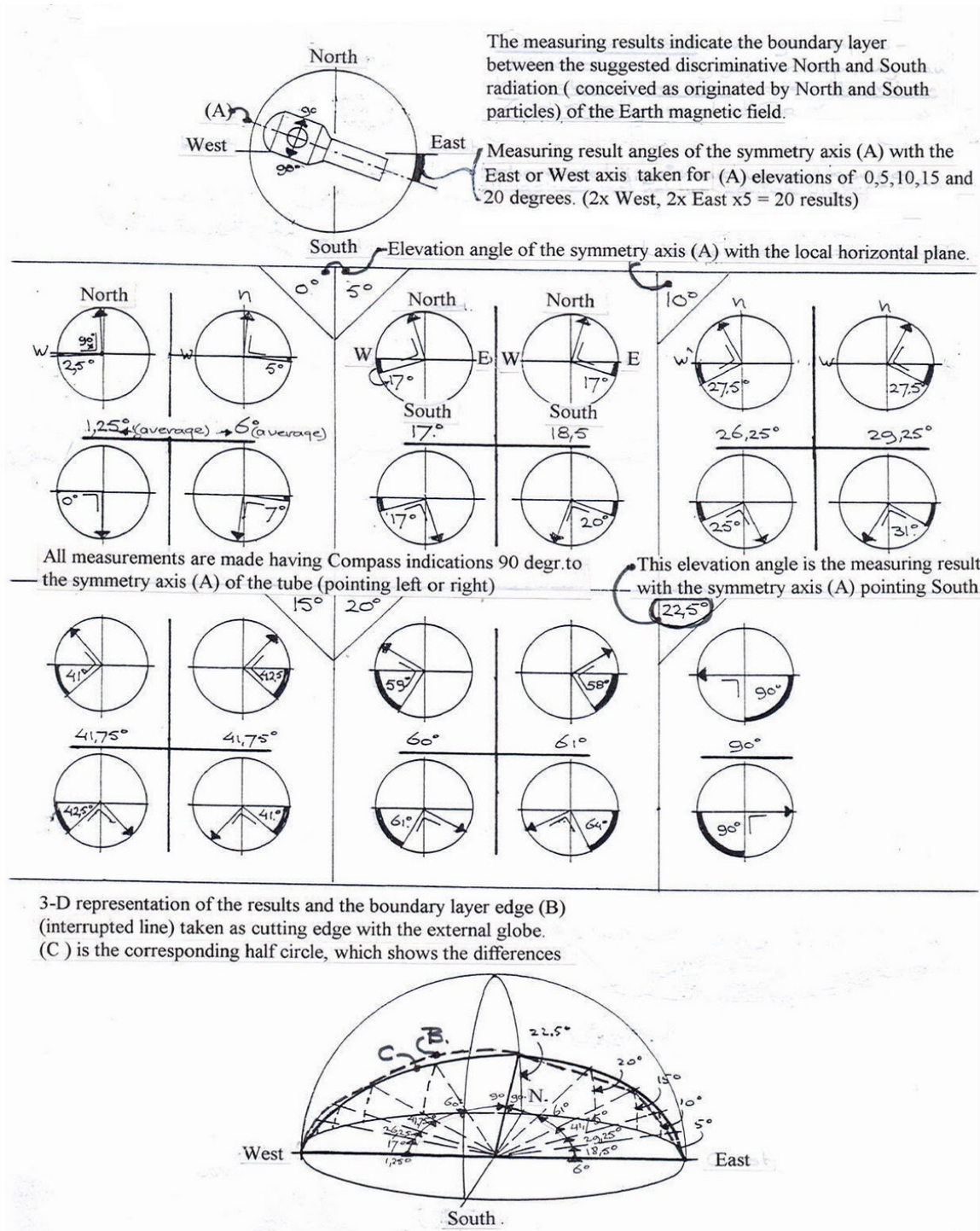
Figure 13, 3-Dimensional representation of the “boundary layer” B, between the North and South monopole radiation of the earth, is the result of multiple measurements by the magnetic telescope at location, Latitude: 52,18 degr. North and Longitude degr. 5,2 East.(see: figure 12).
