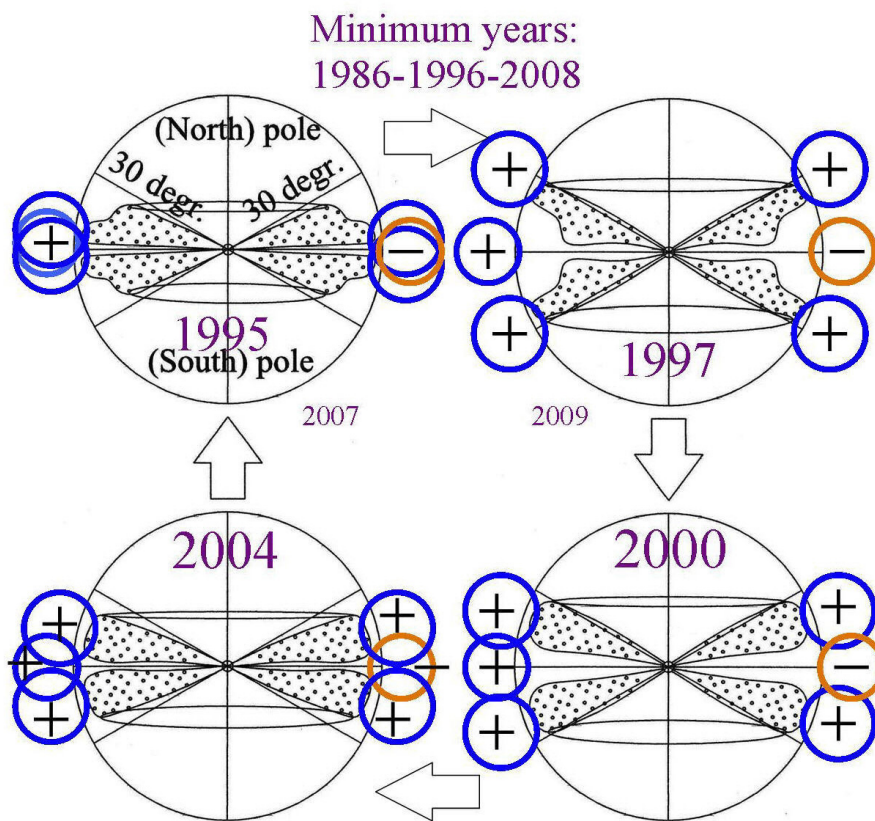
Figure 9 , Cross section through the sun with the sunspot (micro black hole) distribution in two mirror symmetrical double cones, changing shape with the 11 year sunspot cycle. The gravity influence of the double cones together with the solar rotation (blue and yellow ring area) is supposed to be the origin of Solar eclipse gravity variation of the measurements.
