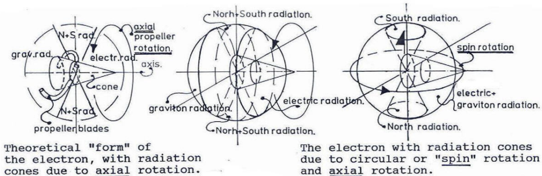
Figure 2, Double axial spin of Fermions with monopole Gluon- Graviton radiation cones. (Ref.3) After a short distance the 5 string shaped Gluons (2 Electric, 2 Magnetic and one general) can merge with Fermions into compound Quarks, or become a photonic wave, just like the Graviton.
