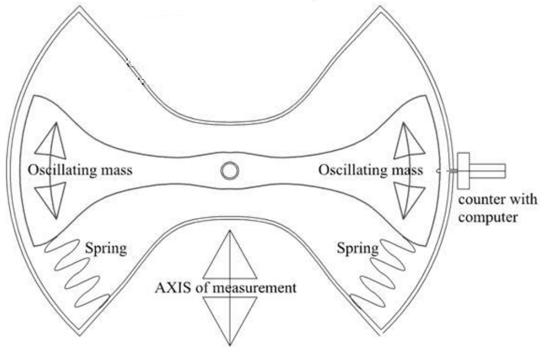
Figure 8 , Cross section through the inertia oscillator for the search of mass concentrations inside the near earth and as a test for double Le Sage gravity.
