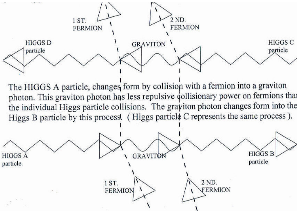
Figure 5, The principle of the Double Le Sage gravity force transfer between two Fermions.
