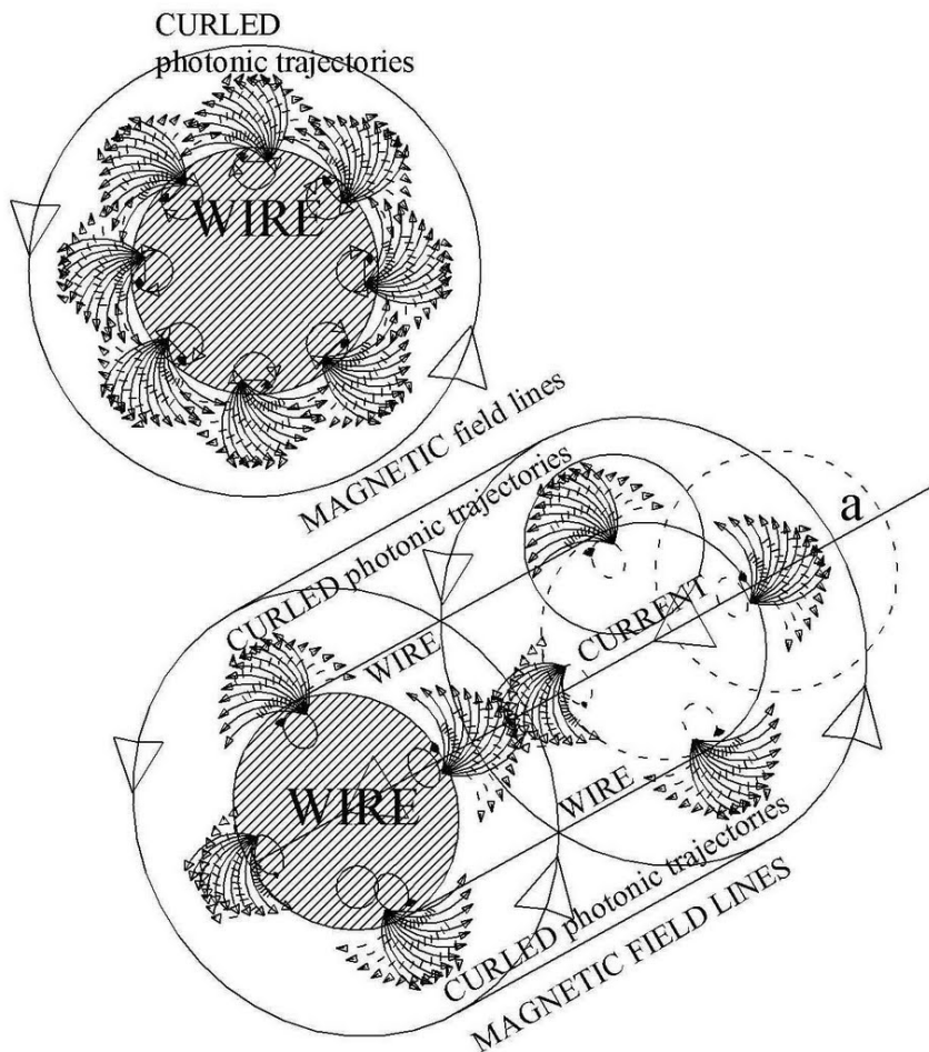
Figure 10, Alternative magnetic field by "curled Photonic monopole information" around an electric wire under current.
