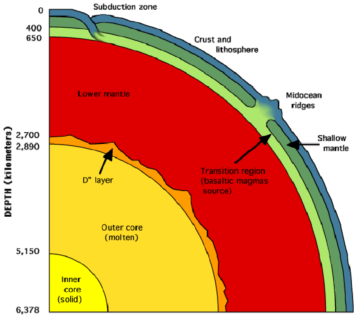
Fig. 1 Internal structure of Earth
