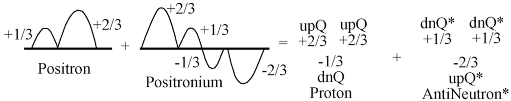
Fig. 4 Possible Proton/Anti Neutron Pair
