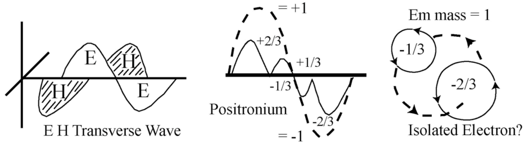
Fig. 1 EH Rad and electron/ positron pairs
