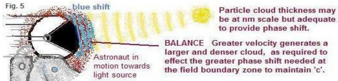
Fig. 5. Doppler shifts at boundaries. The model says that particles behave similarly whether in a small bunch in an accelerator or a large bunch in a galaxy, and anything between. Increased velocity brings an attached thickening cloud of free action particles through which light will propagate at 'c',
