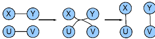
Figure 13.1: Illustration of the reconnection by magnetic flux loops.
