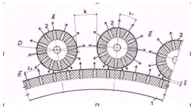
Figure 4.1: Variant of one-ring converter (figure 25 in [36]).
