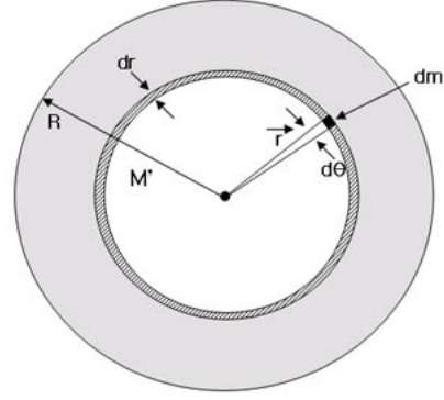
Figure 10: Gravitational self-energy
