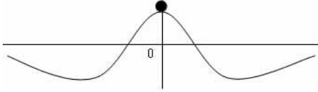
Figure 4: When there is negative mass in potential which has a point of maximum value and a point of minimum value.
