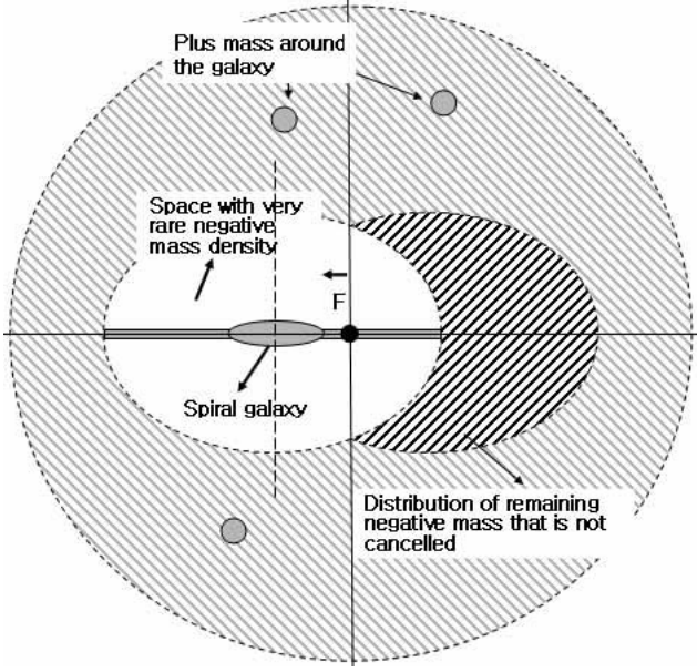
Figure 14: Negative mass effect on arms of galaxy. The actual observed spiral galaxy is on the left. Since repulsive effects occur between negative masses in Newtons dynamics, negative masses will be distributed all over space because it cannot form large mass structures like stars. Negative mass within the galaxy is cancelled out by attraction from large positive mass during the galaxy formation process. Furthermore, the space, other than the galaxy, will maintain the distribution state of negative mass.
