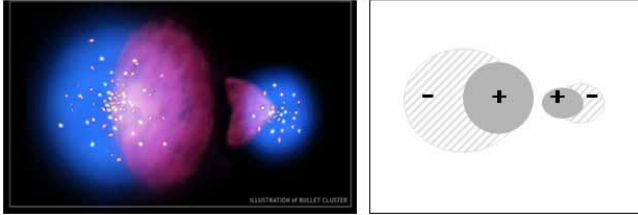
Figure 20: Collision of Bullet Cluster. We can see that general matters(red color) are close to each other, and dark matters(blue color) are on the far side. [18]
