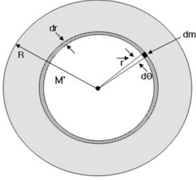
Figure 10: Gravitational self-energy
