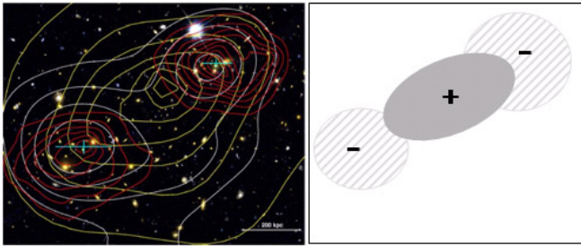
Figure 21: MACS J0025.4-1222 Cluster. We can see that general matters(yellow color) are close to each other(center), and dark matters(red color) are on the far side. [19]
