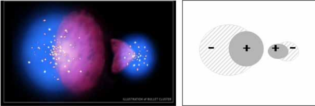
Figure 20: Collision of Bullet Cluster. We can see that general matters(red color) are close to each other, and dark matters(blue color) are on the far side.
