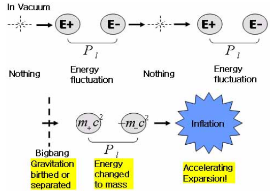
Figure 17: Mechanism of Bigbang and Inflation
