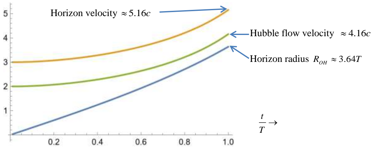
Figure 8.2. 2 A plot of the k = 0.0625 solution with H_0 = 73 \text{ km / sec / Mpc} .
