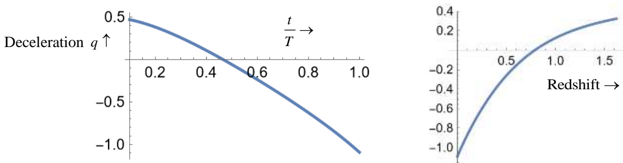
Figure 8.2.3 A plot of deceleration parameter q versus time on the left, and versus redshift z on the right, for the k = 0.0625 solution.
