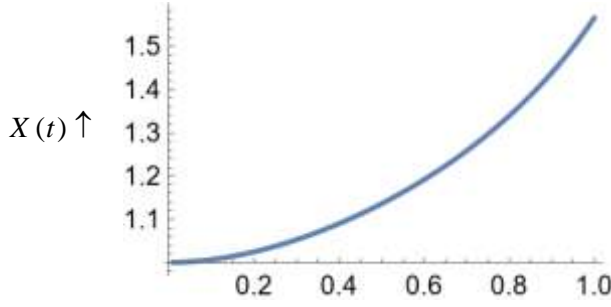
Figure 8.2.6 A plot of X(t) as in Equ's.(8.2.3) & (8.2.13). The massive graviton coupling parameter that increases as the square of the mass ratio of massive gravitons plus baryons, is the above curve squared i.e. X(t)^2 .
