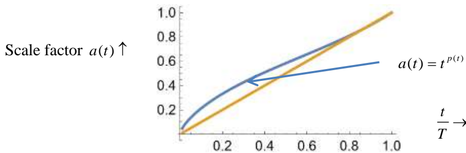
Figure 8.2.4 A plot of the scale factor showing similar behaviour to the Lambda-CDM. All solutions show similar scale factor behaviours.
