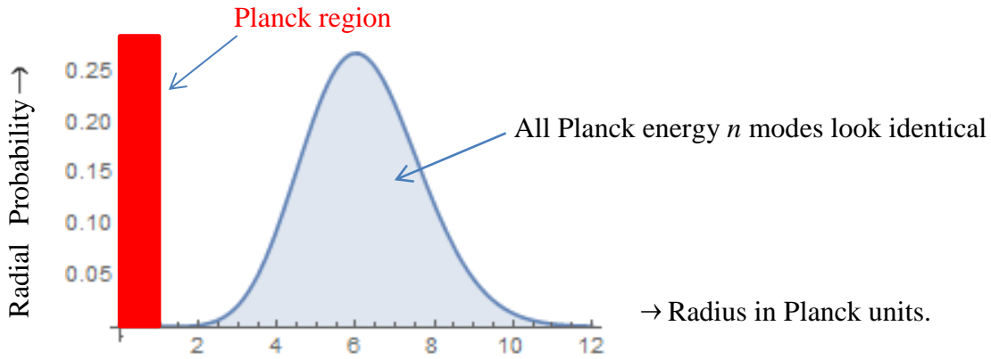
Figure 4.2.1 Plot of radial probability of all n = 3, 4, 5, 6 & 7 Planck energy modes. Despite each mode having Planck energy, the probability in every case of being inside the Planck region is virtually zero at \approx 8.9 \times 10^{-7} .
