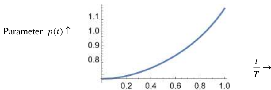
Figure 8.2.5 The of the parameter p(t) for the k = 0.0625 solution.
