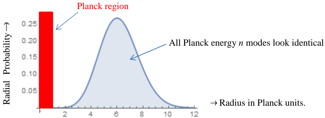
Figure 4.2.1 Plot of radial probability of all n = 3,4,5,6\&7 Planck energy modes. Despite each mode having Planck energy, the probability in every case of being inside the Planck region is virtually zero at \approx 8.9 \times 10^{-7} .
