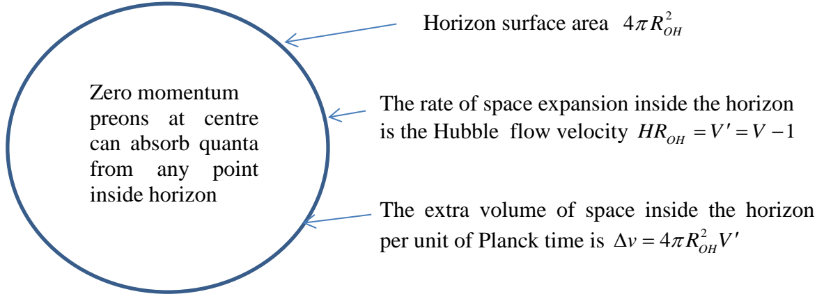
Figure 5.3.1 Preons forming a central mode k are born with zero momentum and infinite wavelength. They can borrow modes from anywhere inside the horizon. The extra volume of space available for this inside the horizon due to the scale factor expansion, can be thought of as a holographic type layer on that horizon that is the Hubble flow velocity V' thick. If V' = 2c for example, this holographic layer is just two Planck lengths.
