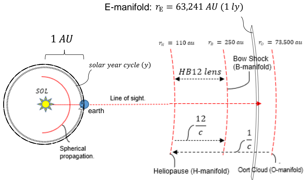
Figure 13: as per based on figure 1, paper 33 ([33]: p9, fig1), the distance of the r_E manifold is calculated using the idea of Earth as a solar year ( y ) reference as one revolution around ol in accompanying the propagation of light from Sol , calculating this value thence as 63,241 AU.
