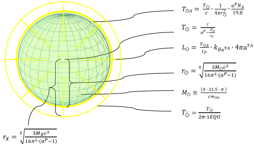
Figure 12: Highlighting the phenomenal features of Sol from the derived fine structure constant ( \alpha ) and Planck ( h ) values.
