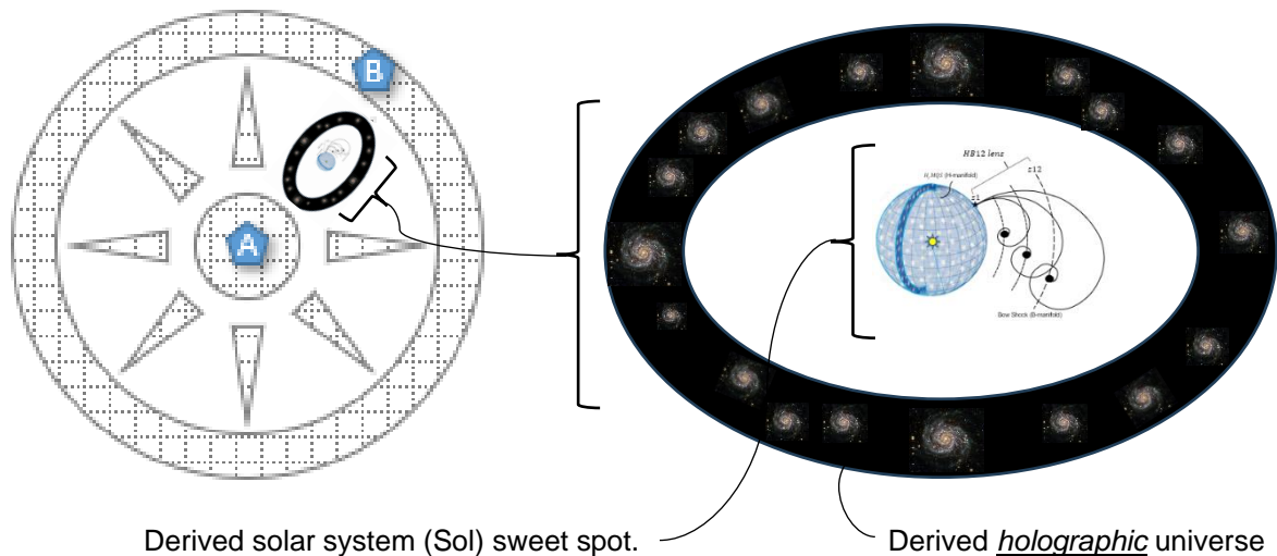
Figure 15: ( not drawn to temporal or spatial scale ) the universal “sweet spot”, noting the zero-dimensional number theory correctly derived the “non-existence” feature of the universe (as a hologram in this case) given the zero-dimensional number theory takes the context of the moment at the big bang.
