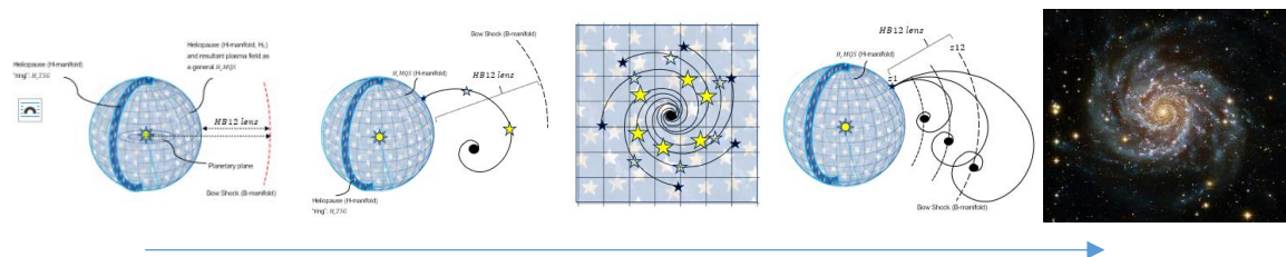
Figure 14: r_H TSG and associated HB12 scheme from paper 33 ([33]: p13-16, fig4-8)
