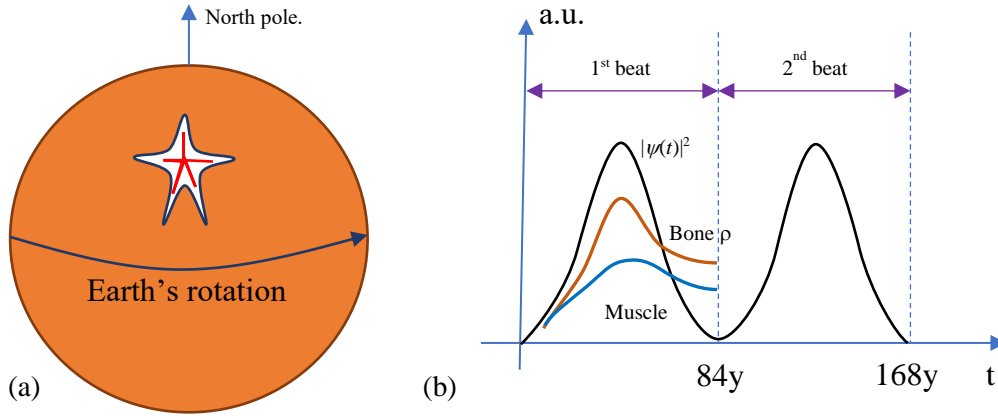
Fig.7 (a)A human sketch with the head pointing to the North Pole. (b) the biological clock.
