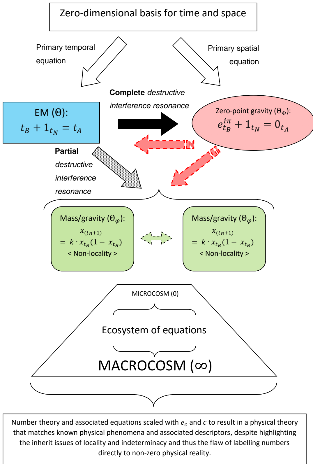
Figure 5: An overall schematic of the relationship between the proposed zero-dimensional number theory and physical phenomena.
