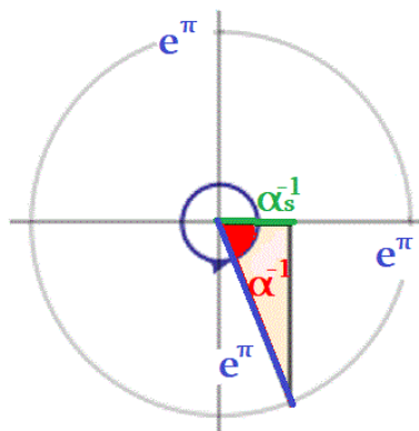
Figure 2. The angle in \alpha^{-1} radians. The rotation vector moves in a circle of radius e^n .
