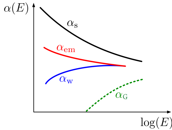
Figure 14. Variation of the coupling constants of the four fundamental interactions of physics as a function of energy.
