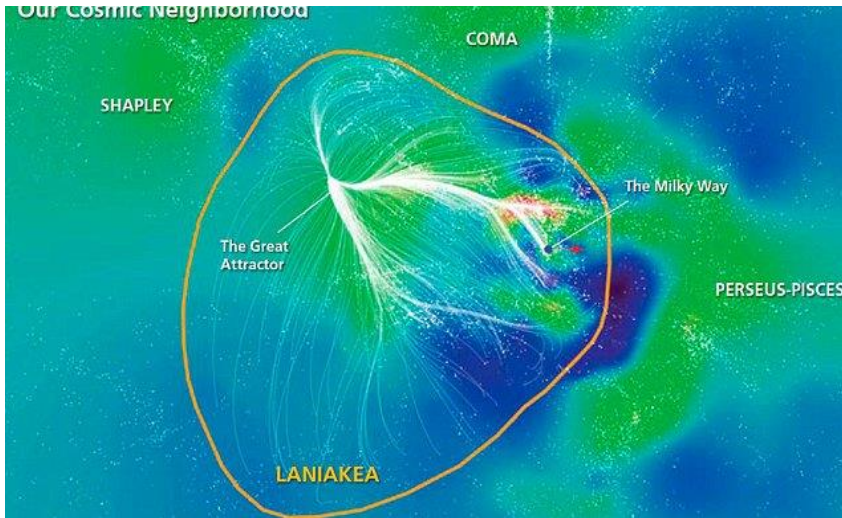
Figure 1. Laniakea Supercluster. Adapted from [Tully, R. B., et al. (2014) The Laniakea supercluster of galaxies. Nature , 513 , 71. arXiv:1409.0880].
