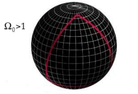
Figure 16. If \Omega_0 is greater than 1, the Universe is closed and this will eventually halt its expansion and recollapse.
