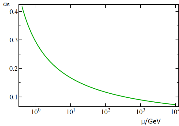
Figure 1. Strong coupling constant \alpha_s as a function of the energy.
