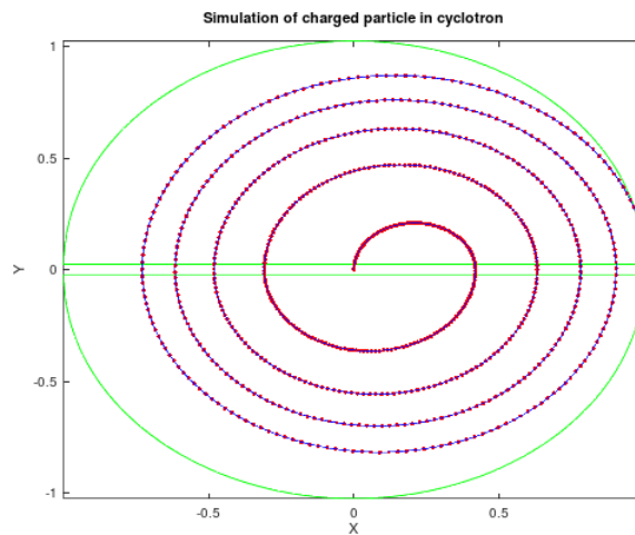
Figure 2: Simulating the trajectory of electron
