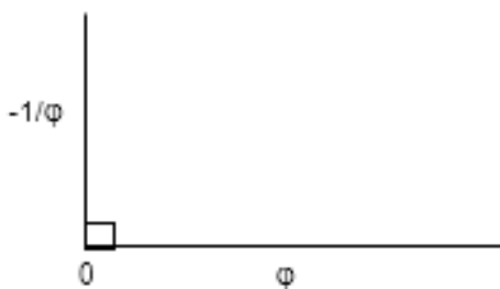
Figure 1: two axes of time, \frac{-1}{\varphi} and \varphi ,
