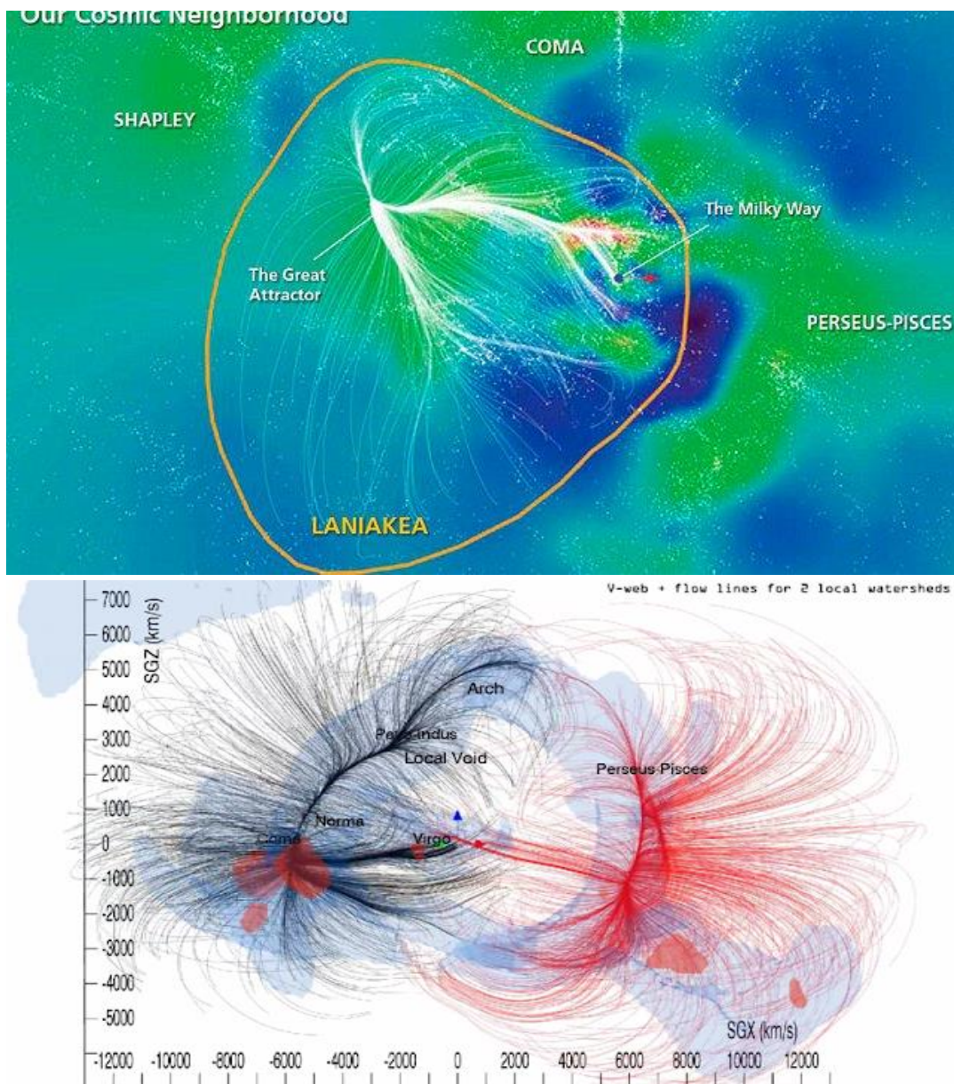
Fig. 2. A representation of structure and flows due to mass within 6,000 \text{ km s}^{-1} ( \sim 80 \text{ Mpc} ). Surfaces of red and blue respectively represent outer contours of clusters and filaments as defined by the local eigenvalues of the velocity shear tensor determined from the Wiener Filter analysis. Flow threads originating in our basin of attraction that terminate near the Norma Cluster are in black and adjacent flow threads that terminate at the relative attractor near the Perseus Cluster are in red. The Arch and extended Antlia Wall structures bridge between the two attraction basins. Adapted from [28].
