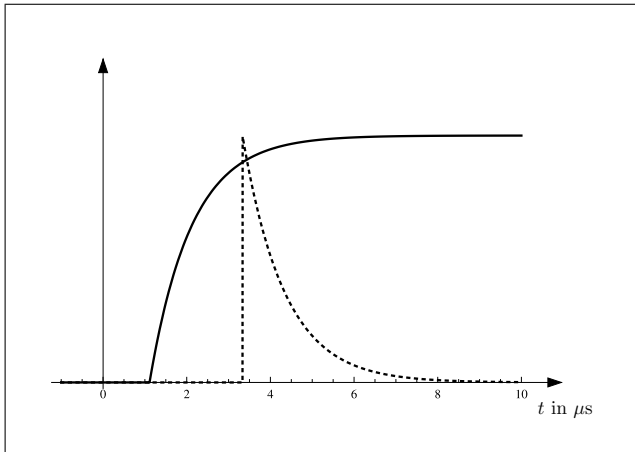
Fig. 3. Parts of the signal (39) at x = 1000\text{m} for \tau = 1\mu\text{s} and u = 3c .
