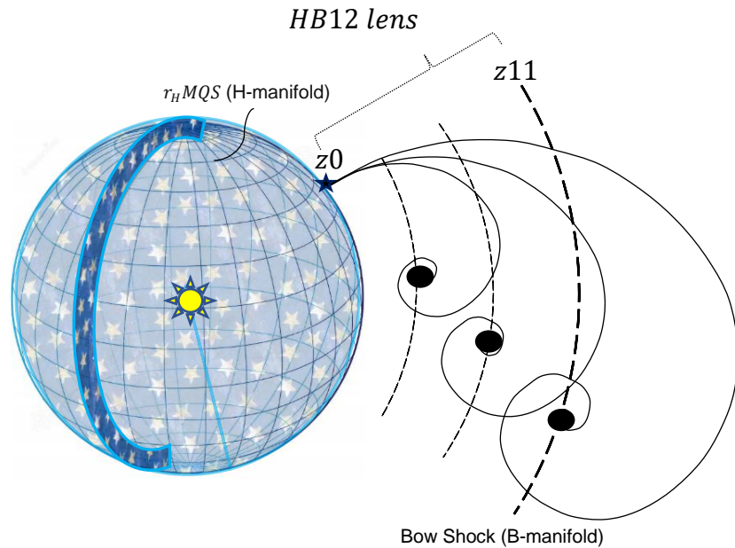
Figure 7: Depiction of various sized HB12 time-space circuits extending to varying depths and therefore varying redshifts according to their depth to the Bow Shock, from a redshift of z_0 to z_{11} .
