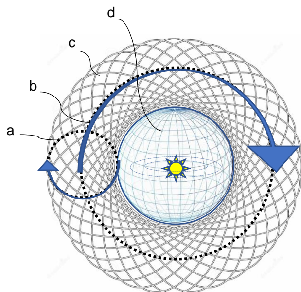
Figure 2: View of a time-space circuit torus as though from the side of solar system planetary plane; a time-space circuit circle between the O-Manifold and H-Manifold (a), a time-space circuit ring (b) in the region between the O-Manifold and H-Manifold, the general fixed pattern effected by the O-Manifold (c), and the amplified H-Manifold (d) by the effect of the connection via (a) with the O-Manifold.
