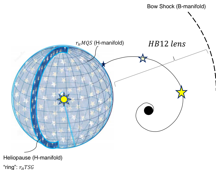
Figure 5: depiction of a HB12 time-space circuit spiral, from a region of minimal to no illumination, to then greater illumination, to an ultimate exhaustion-point of illumination (black dot).
