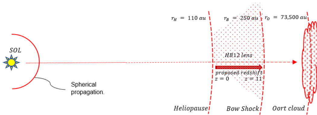
Paper 32, Figure 2: a universal scale from a source of light as the Sun outwards in a spherical wavefront of light a distance of r_O = 73,500 \text{ au} , tracked back a time-scale measurement of “c” to the Heliopause as r_H = 110 \text{ au} , while then factored by “12” upon the r_H level to arrive at r_B , the proposed Bow Shock manifold.
