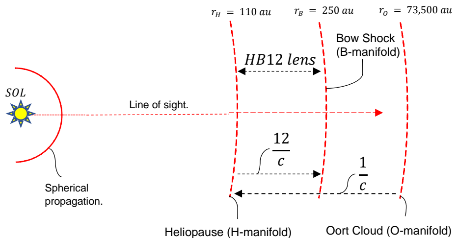
Figure 1: Attributing new “manifold” terms for the Heliopause (H-manifold), Bow shock (B-manifold), and Oort Cloud (O-manifold), the Oort Cloud as the prescribed Epoch of time-space, and highlighting the \frac{1}{c} and \frac{12}{c} features of the HB12 lens region.
