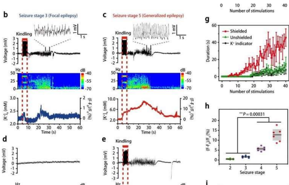
a, In vivo experimental scheme for external potassium concentration sensing in a kindling-induced epileptic mouse model, in which repeated electrical stimulations increases the seizure severity. b-e, Simultaneous neural activity recording and fluorescent imaging of the mice at different epileptic seizure stages (b: seizure stage 3; c: seizure stage 5). Credit: IBS
