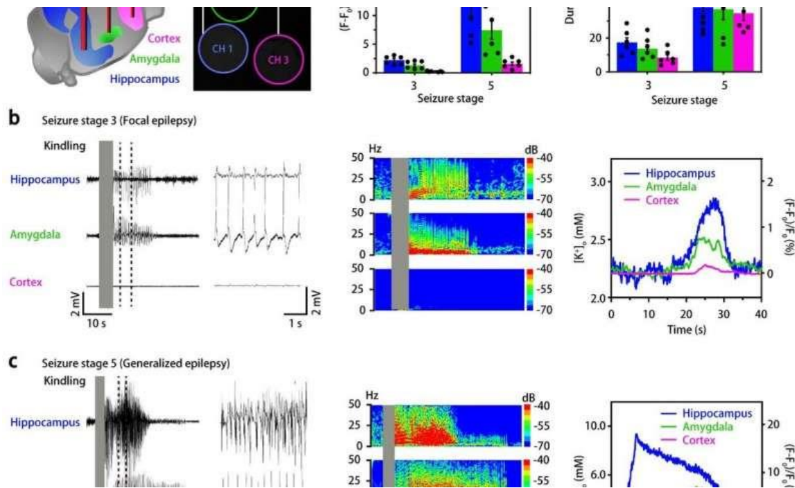
a, Experimental scheme for simultaneous electroencephalography (EEG) recording and K^+ sensing in three different brain regions (hippocampus, amygdala, and cortex) of the epileptic mouse. b, c, Upon electrical stimulation of the hippocampus that resulted in different degrees of epileptic seizures, both the EEG recording and the nanosensor data show responses in amygdala and cortex. d, e, Graphs showing the seizure stage-dependent changes in the amplitude (d) and duration (e) of the nanosensor fluorescence signal in the three different locations of the mouse brain. Credit: IBS
