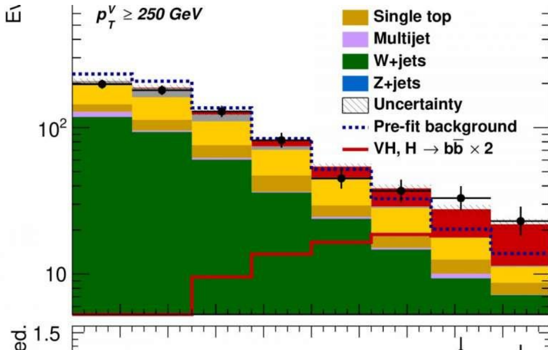
Figure 2. Observed and predicted distribution for one of the 14 BDTs used to separate the Higgs boson signal from the background processes. The Higgs boson signal is shown in red, the backgrounds in various colours. The data points are shown as points with error bars. Credit: ATLAS Collaboration/CERN
