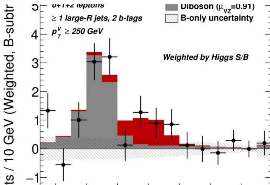
Figure 3: A comparison of the excess of collision data (black points) over the background processes (subtracted from the data). Shown are the reconstructed mass from the H \rightarrow bb decays (red) and the well-understood diboson Z \rightarrow bb decay (grey) used to validate the result. Credit: ATLAS Collaboration/CERN
