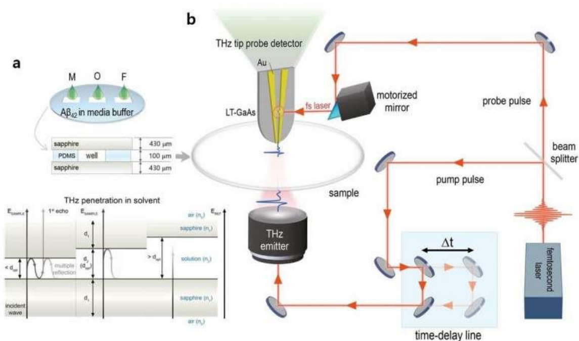
Figure 2. Experimental setup. (a) Samples of the A \beta proteins in monomer (M), oligomer (O) and fibril (F) form are analysed inside small wells sandwiched by sapphire plates. With a small amount of sample, it was possible to detect THz signals without noise. (b) Solution-based sample preparation for the THz near-field time-domain spectroscopy system. Credit: Institute for Basic Science
