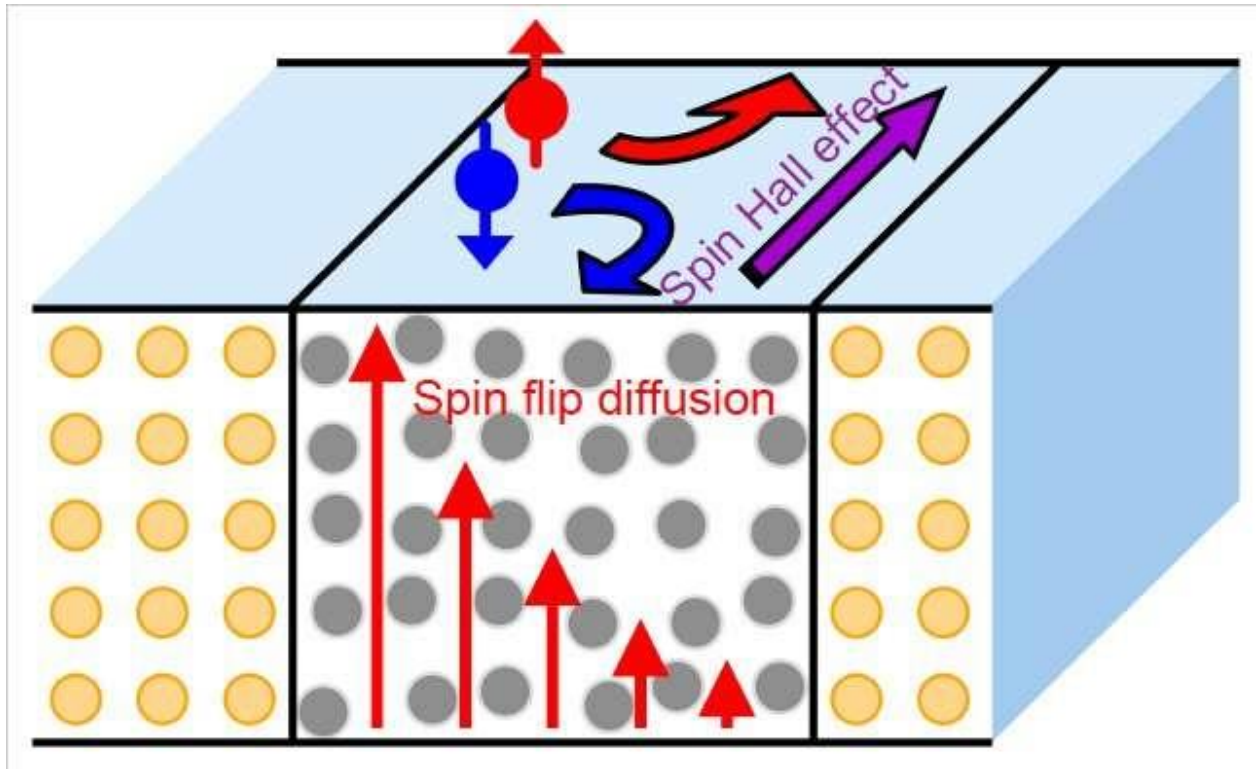
Figure explaining the Spin Hall Effect. Credit: Gupta et al.
